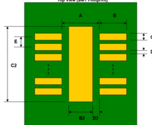
Top View (SMT Footprint)
